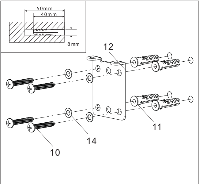
Concrete Wall
