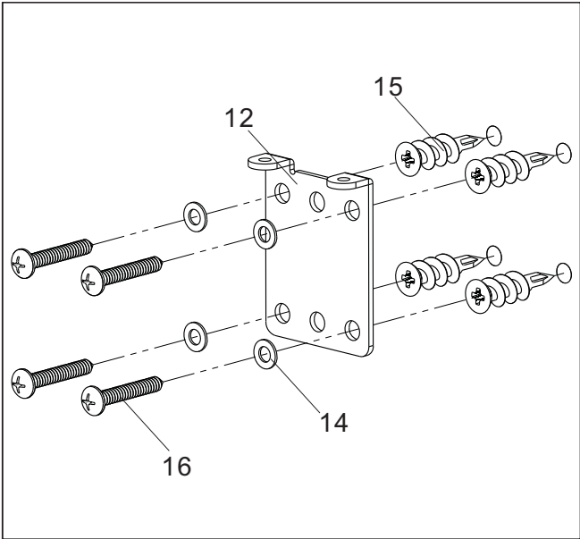
Dry Wall
