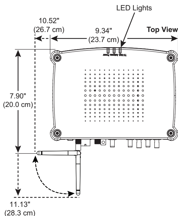
Figure 7: TV-Hub Dimensions - Vertical Orientation
