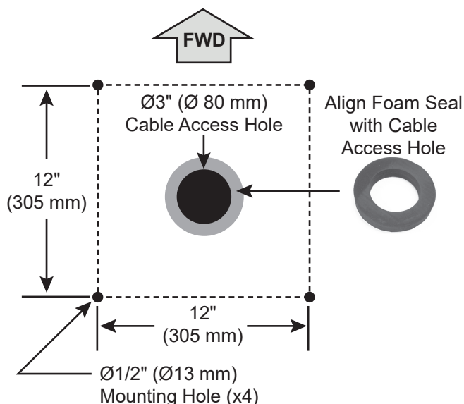
Figure 8: Antenna Mounting Holes Layout
