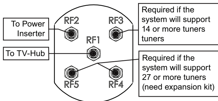
Figure 15: Connectors on Bottom of Antenna
