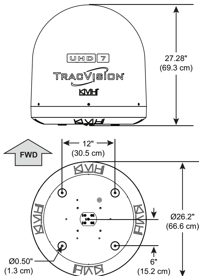
Figure 5: Antenna Dimensions
