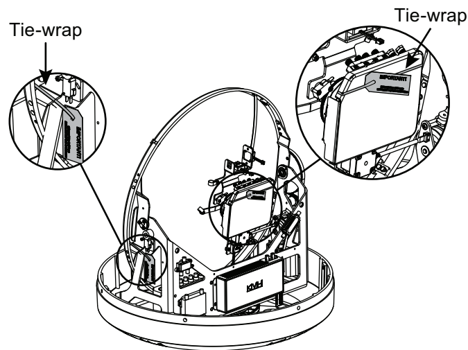
Figure 18: Antenna Restraints
