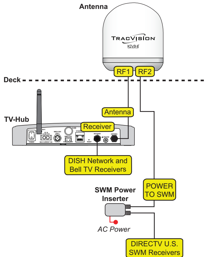
Figure 22: Receiver/DVR Wiring
