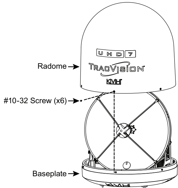
Figure 11: Shipping Restraints
