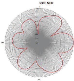
E-Plane Pattern
