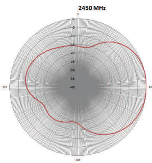
E-Plane Pattern
