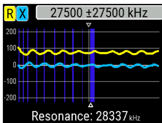
Example 2: Unknown cable
