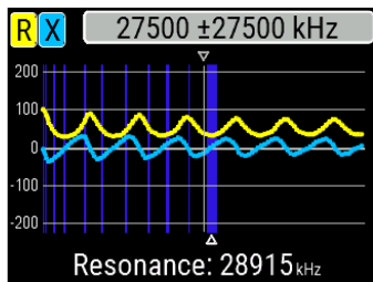
Example 1: 50-Ohm cable
